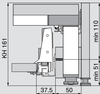
Space requirements in the cabinet
