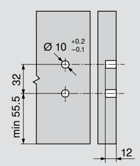
Front drilling distances for EXPANDO
