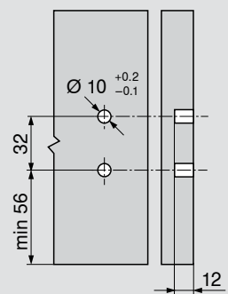
Front drilling distances for EXPANDO
