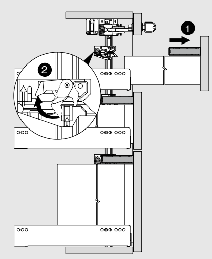
Pull-outs
