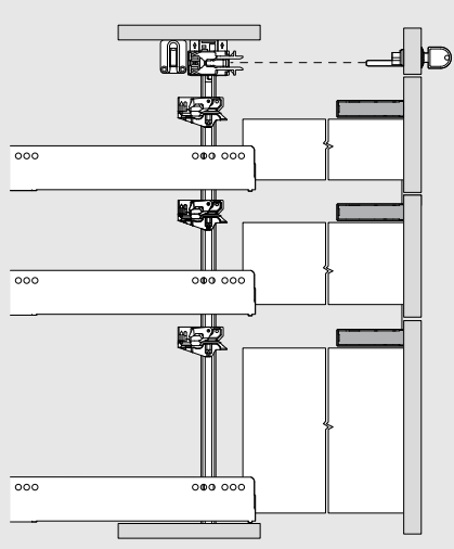
Pull-outs
