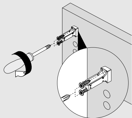
Front piece for front locking bracket
