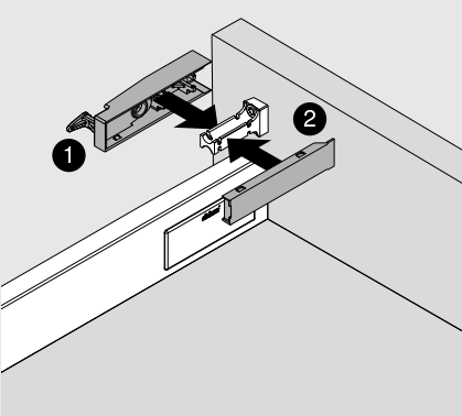
Front locking bracket and cover cap
