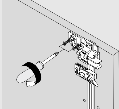
Attachment for synchronisation
