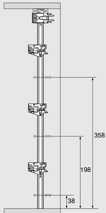
Fixing position of cabinet profiles
